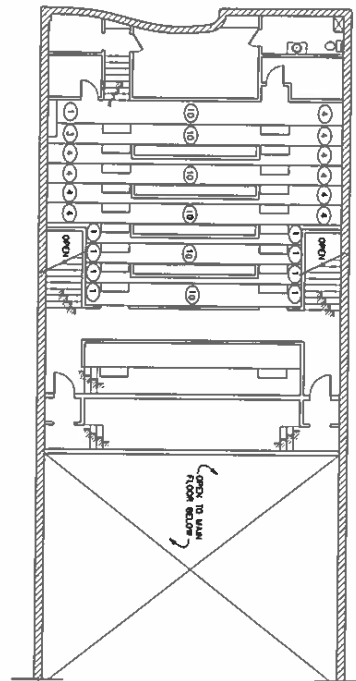
2 UPPER LEVEL AUDITORIUM PLAN 1/8" = 1'-0"
